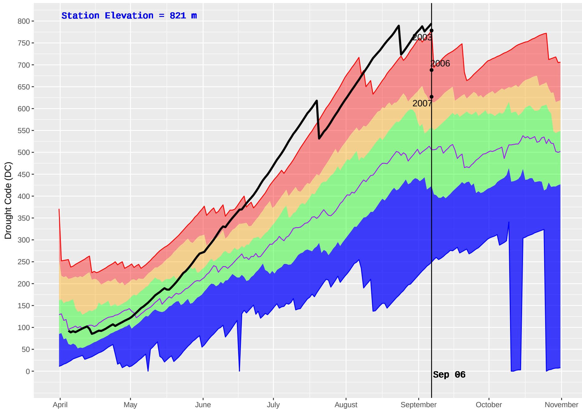
KNIFE (225) : Historical (1991–2016) and Current (2017) Noon Drought Code (DC)
