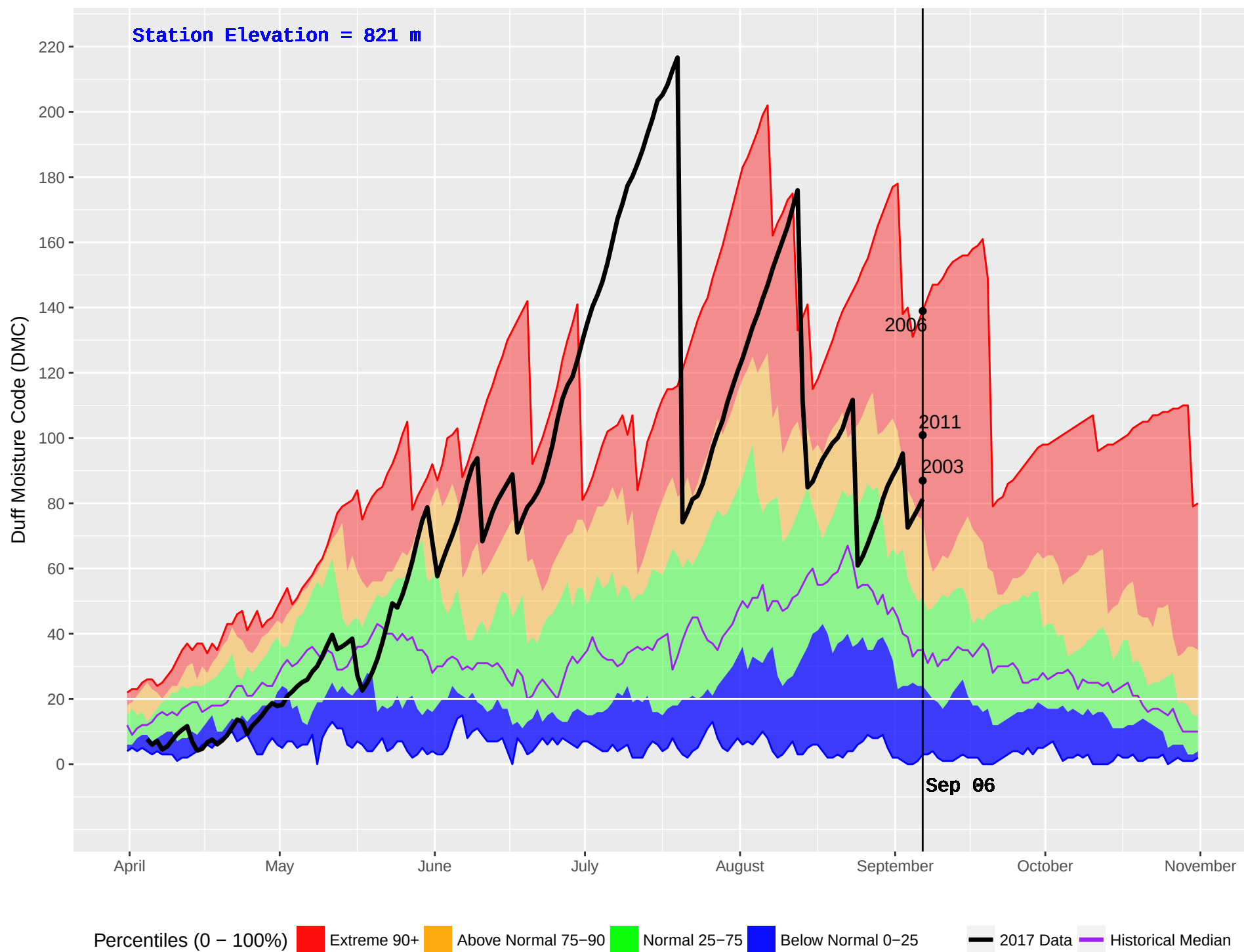
KNIFE (225) : Historical (1991–2016) and Current (2017) Noon Duff Moisture Code (DMC)
