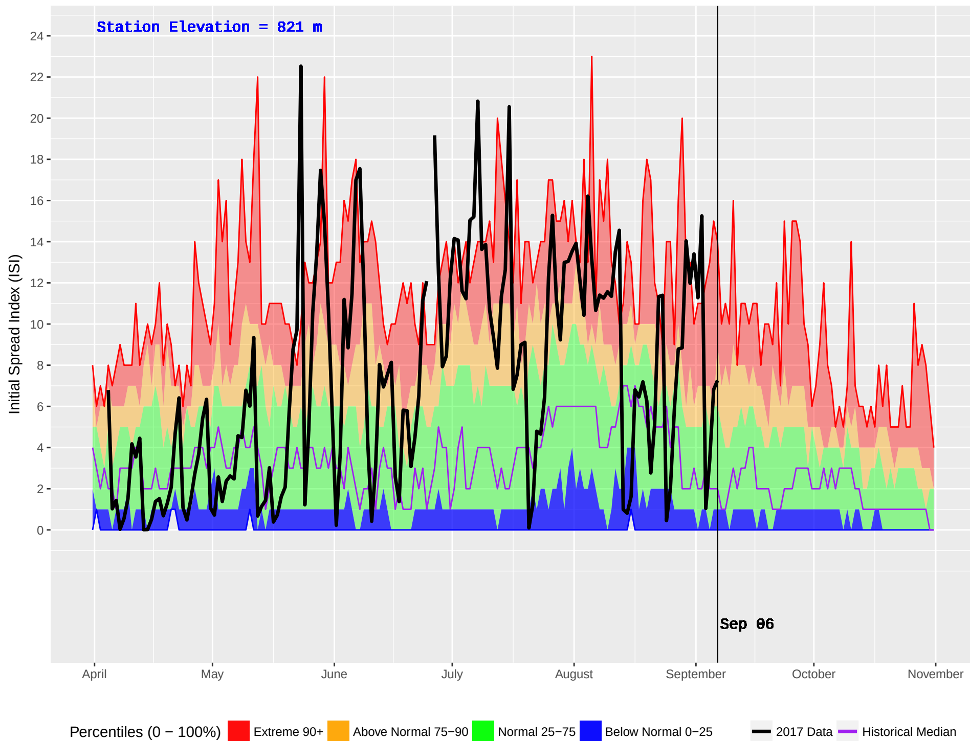
KNIFE (225) : Historical (1991–2016) and Current (2017) Noon Initial Spread Index (ISI)
