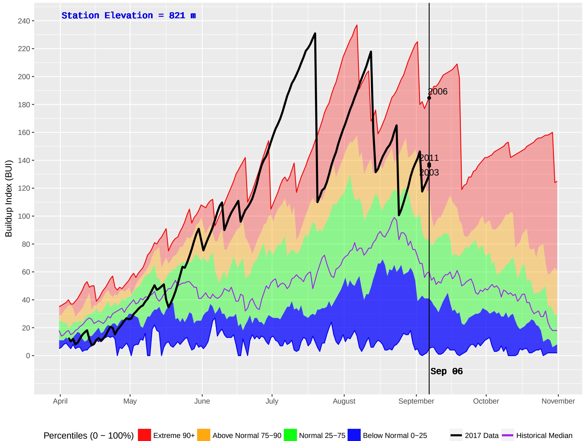
KNIFE (225) : Historical (1991–2016) and Current (2017) Noon Buildup Index (BUI)
